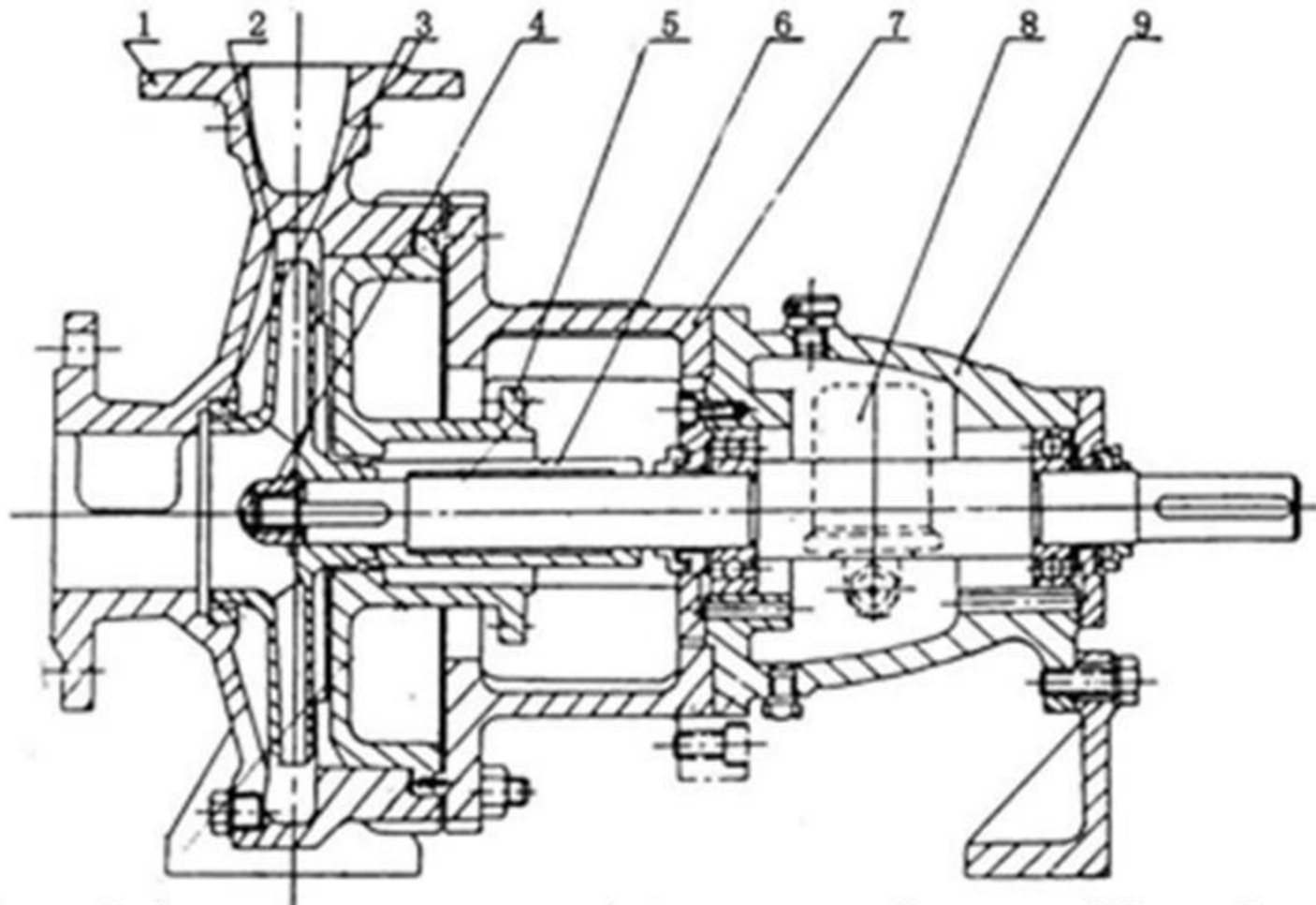
1.Pump Casing 2.Impeller 3.Seal-ring 4.Impeller Nut 5.Pump Cover 6.Seal Part 7.Mid.Bracekt 8.Shaft 9.Hanging stand
